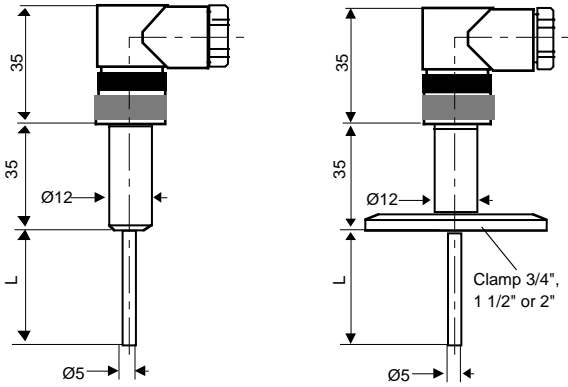
P2209 with IEC 947-5-2 plug
