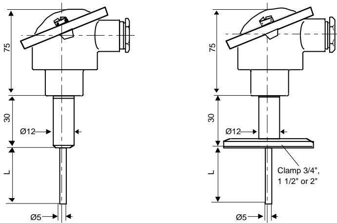
P2209 with built-in transmitter
